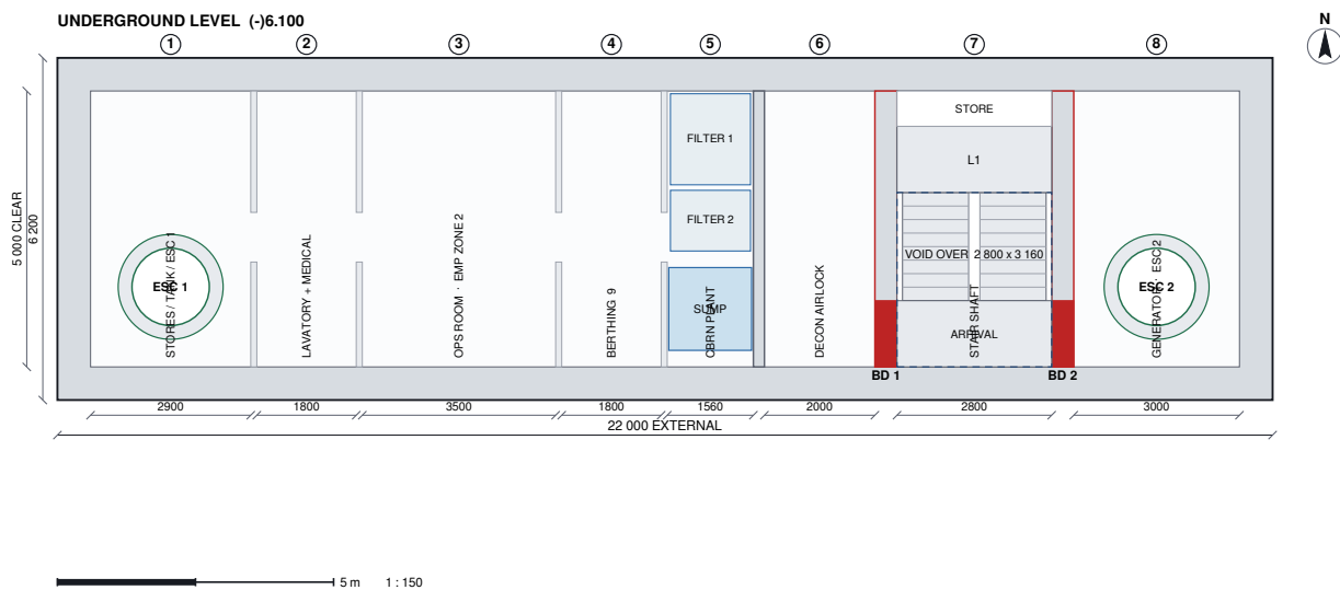
Fig 3.1 : Underground Level Plan at (-)6.100
