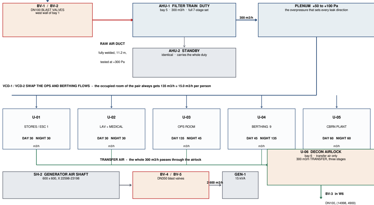
Fig 10.2 : Ventilation Air Path and Room Distribution
